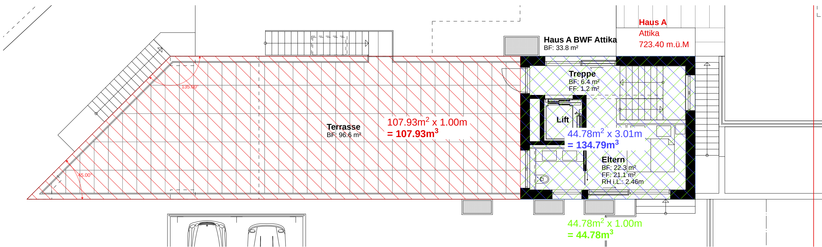
Attika
